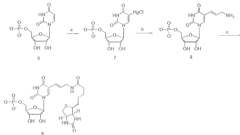
SCHEME 2 Attempted synthesis of the biotinylated monophosphate 9. Conditions: (a) \text{Hg}(\text{OAc})_2 , LiCl, NaOAc, pH 6 buffer; (b) (1) trifluoroacetyl allylamine, \text{K}_2\text{PdCl}_4 , NaOAc buffer, DMF, 80^\circ\text{C} , 2 hours; (2) \text{NH}_4\text{OH} , RT; (c) biotin N -hydroxysuccinimide, pyridine, \text{Et}_3\text{N} .
