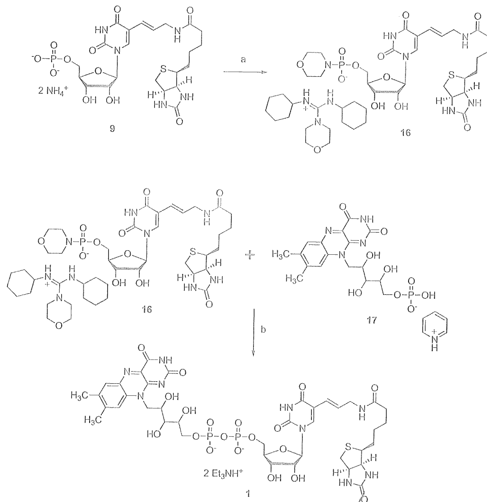
SCHEME 5 Synthesis of the pyrophosphate 1. Conditions: (a) DCC, morpholine, t -BuOH, H 2 O, reflux, 4 hours (52%); (b) triethylamine, pyridine, tetrazole, RT, 6 days (5%) or MnCl 2 , Na 2 SO 4 , formamide, RT, 18 hours (10%).
