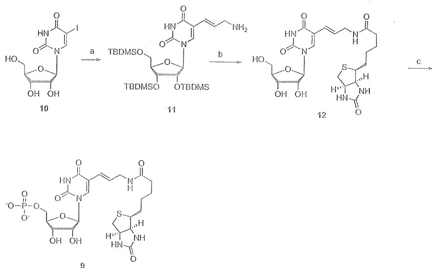
SCHEME 3 Synthesis of the monophosphate 9 with partial protection. Conditions: (a) (1) trifluoroacetyl allylamine, Na 2 PdCl 4 , NaOAc buffer, DMF, 80°C, 2 hours; (2) TBDMSCl, imidazole, DMF; (3) NH 4 OH, MeOH, RT, 17 hours (40% for 3 steps); (b) (1) biotin N -hydroxysuccinimide, pyridine, Et 3 N, RT, 2 hours; (2) Et 3 N·3HF, THF, RT (75% for two steps); (c) triethylphosphate, POCl 3 , H 2 O, 0°C, 18 hours, (45%).
