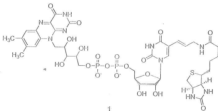
FIGURE 2 The chemical structure of the pyrophosphate with a biotin tag.
