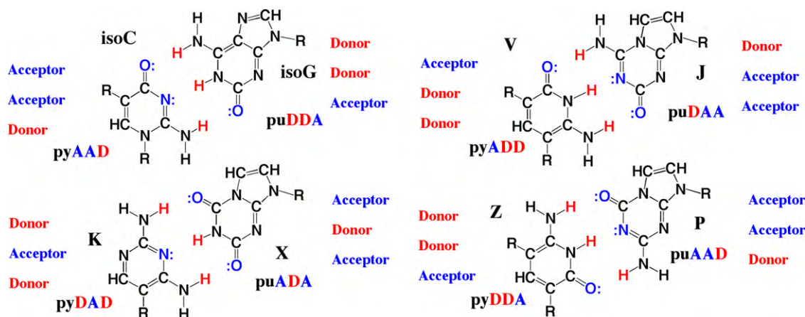
Fig. 8. Shuffling hydrogen bond donor and acceptor groups in the standard nucleobase pairs generated eight additional heterocycles that, according to simple theory, should form four new, mutually independent, base pairs. This is called an “artificially expanded genetic information system” (AEGIS). Could molecular behavior at the center of genetics and Darwinian Evolution be so simple? Synthesis was used to decide.
