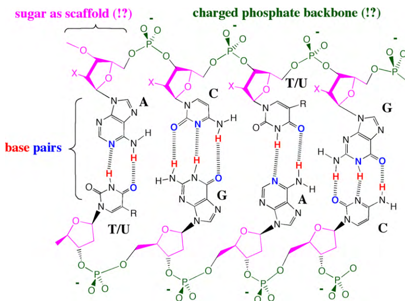
Fig. 3. The rules governing the molecular recognition and self-assembly of DNA duplexes are so simple that many are tempted to believe that molecular recognition in chemistry is, in general, similarly simple. Hence, various individuals seek “codes” for protein folding or drug binding.
