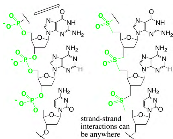
Fig. 6. The repeating backbone anion drives the interaction between two strands as far from the backbone as possible. This guides strand-strand interactions, and forms the basis for Watson-Crick pairing rules.
