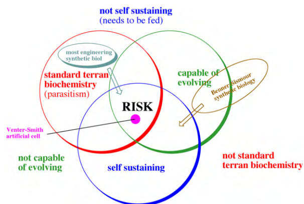
Fig. 12. A Venn diagram illustrating the hazards of synthetic biology. The green circle contains systems able to evolve. Those outside the circle cannot, and present no more hazard than a toxic chemical. The blue circle contains systems that are self-sustaining. Those inside the circle “live” without continuing human intervention; those outside require continuous feeding, and are no more hazardous than a pathogen that dies when released from a laboratory. Systems within the red circle use standard terran molecular biology; those outside do not. The greatest chance for hazard comes from a system that is self-sustaining, uses standard biochemistry, and is capable of evolving, the intersection between the three circles.
