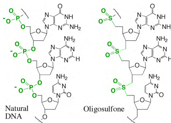
Fig. 5. Replacing phosphates (–PO 2 – units, each having a negative charge, left) in DNA by dimethylenesulfone linkers (the –SO 2 – units, right, each lacking a negative charge) gave an uncharged analog of DNA. The uncharged analog of RNA was also synthesized.
