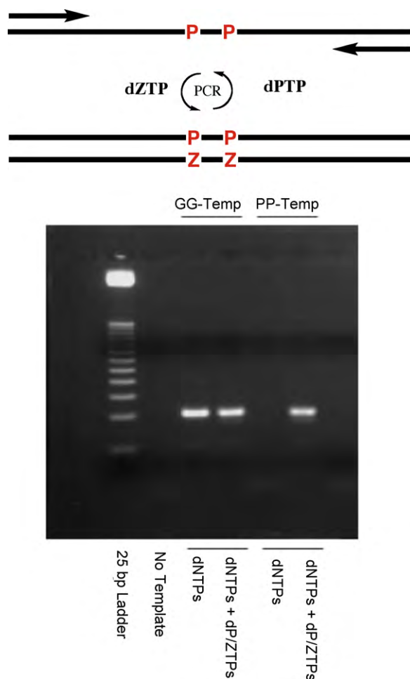
Fig. 11. The polymerase chain reaction with a six-letter genetic alphabet, incorporating P and Z in addition to A, T, G, and C.
