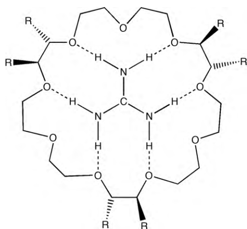
Fig. 1. Synthesis in biology was first used to help understand the connection between biomolecular structure and behavior by making unnatural molecules that bind to small molecules. This synthetic receptor was created by Jean-Marie Lehn and his colleagues to mimic the ability of natural receptors to bind to small cationic ligands, and was cited in his Nobel Prize lecture.
