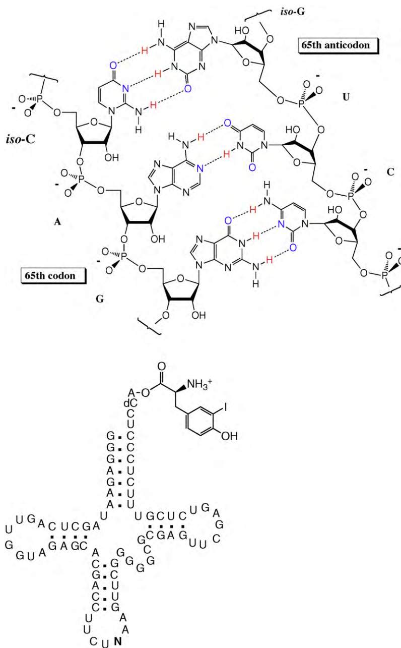
Fig. 9. Putting a synthetic base into a messenger RNA, and providing a transfer RNA having the complementary non-standard base in the anticodon loop (the “N”) allowed the incorporation of a 21st amino acid (here, iodytyrosine) into a protein.
