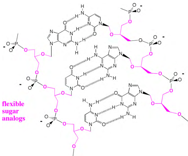
Fig. 4. The failure of these flexible glycerol DNA molecules led us to re-evaluate our view of the role of sugars in double helix formation.
