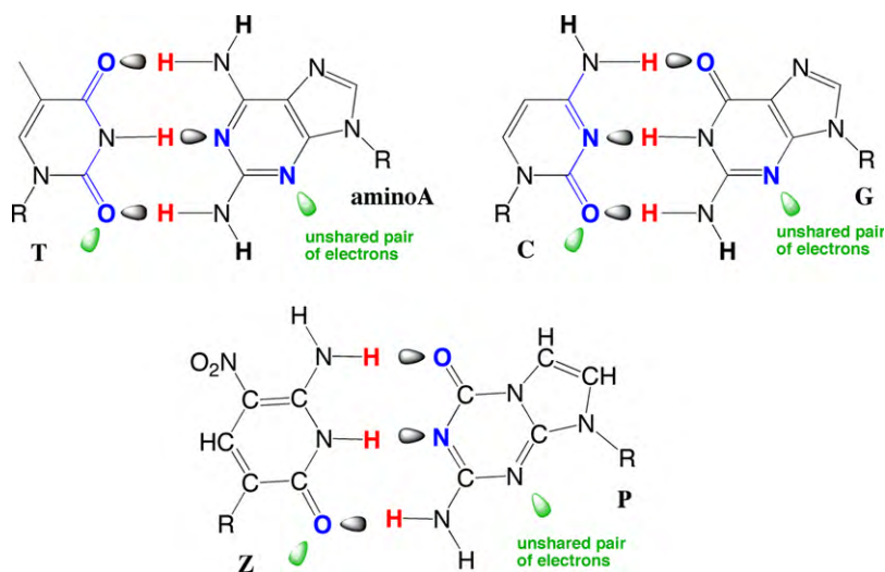
Fig. 10. The Z and P pairs that have been incorporated into six-letter PCR, with mechanistic studies that show that this six-letter synthetic genetic system can support Darwinian evolution. Key to meeting this challenge was to make a small accommodation to the desire of natural DNA polymerases to have nucleobases that present electron density (the green lobes) to the minor groove (down, in this structure) of the double helix. This is the case for T, A (shown here with an extra \text{NH}_2 unit), C, and G (top). It is also the case with the Z and P synthetic nucleobases (bottom).
