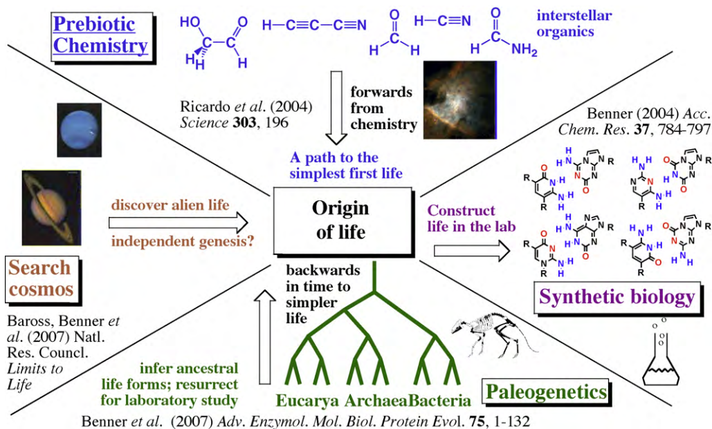
Fig. 2. Four approaches to understand life as a universal.
